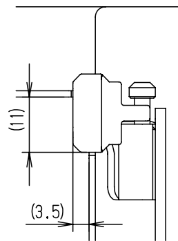
C部詳細 (1:1)
