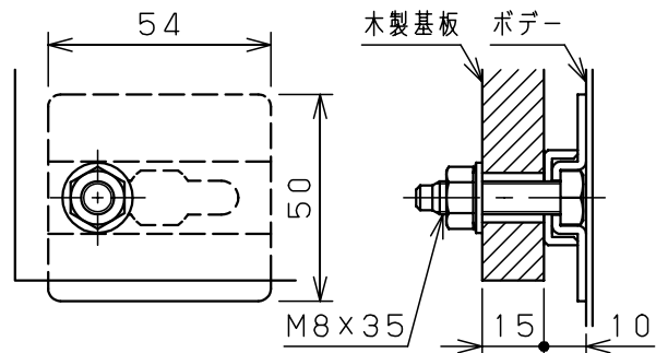
C部基板取付部詳細 (1:2)
